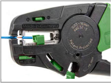
Partially stripping a conductor.
