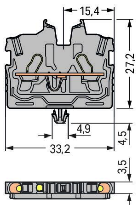
Modular terminal blocks and terminal strips with snap-in mounting feet
