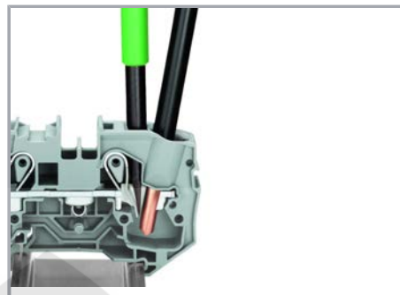
Removing a solid conductor.
