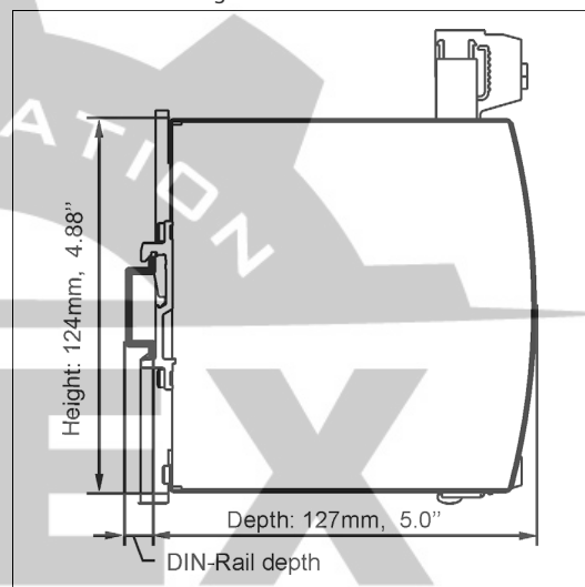
Fig. 17-2 Side view
