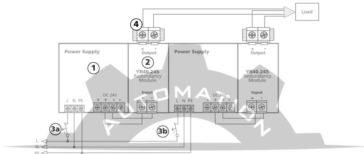
Fig. 7-1 Replacing the power supply or redundancy module while the system is running
