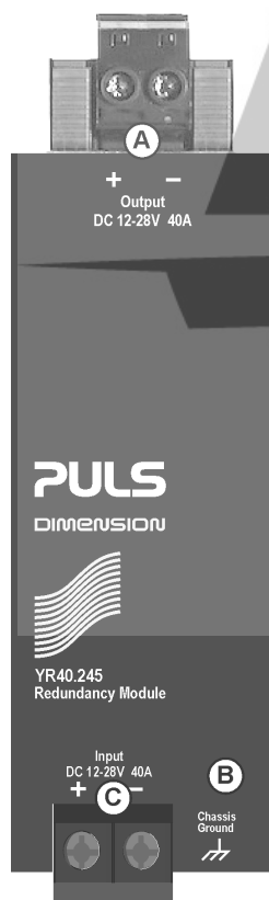
Fig. 9-1 Front side
