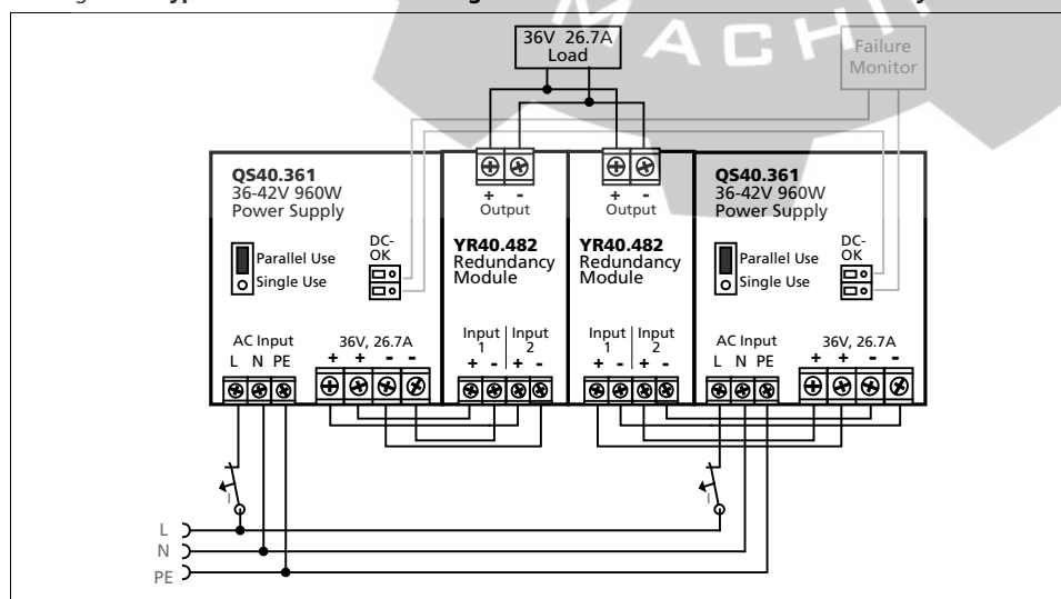
Fig. 25-1 Typical 1+1 Redundant configuration for 26.7A with a dual redundancy module
