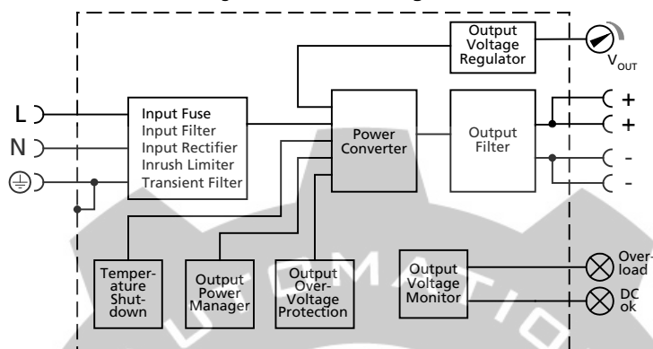
Fig. 10-1 Functional diagram
