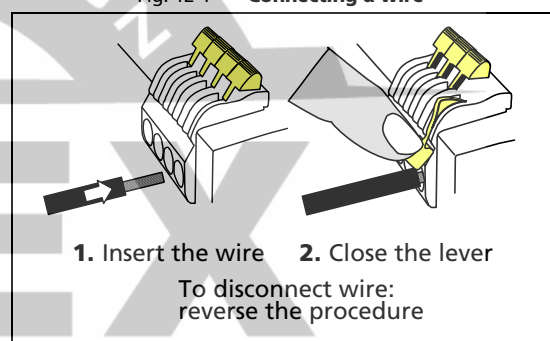
Fig. 12-1 Connecting a wire
