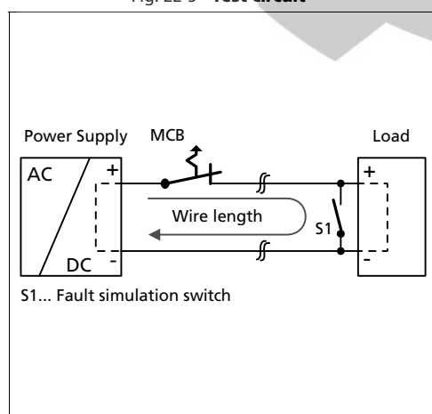
Fig. 22-5 Test circuit
