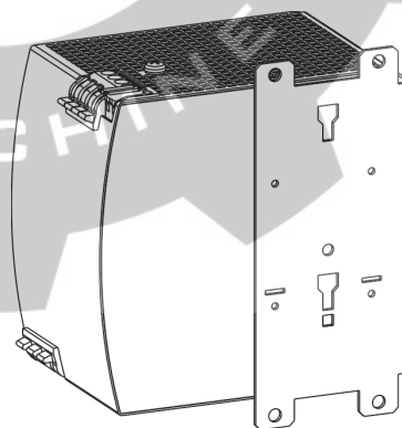
Side mounting without DIN-rail brackets
