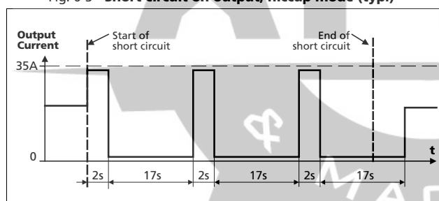
Fig. 6-3 Short-circuit on output, hiccup mode (typ.)
