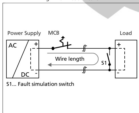
Fig. 22-5 Test circuit
