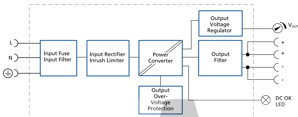
Fig. 11-1: Functional diagram
