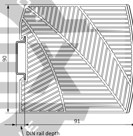
Fig. 20-2: Side view
