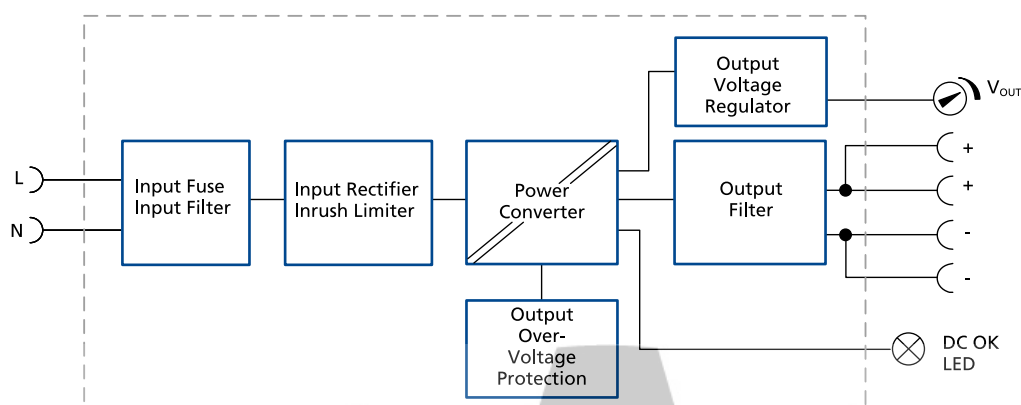
Fig. 11-1: Functional diagram
