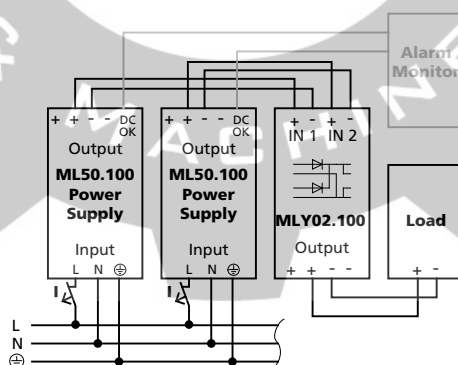
Fig. 17-1 Wiring diagram, 1+1 Redundancy, 2.1A output current
