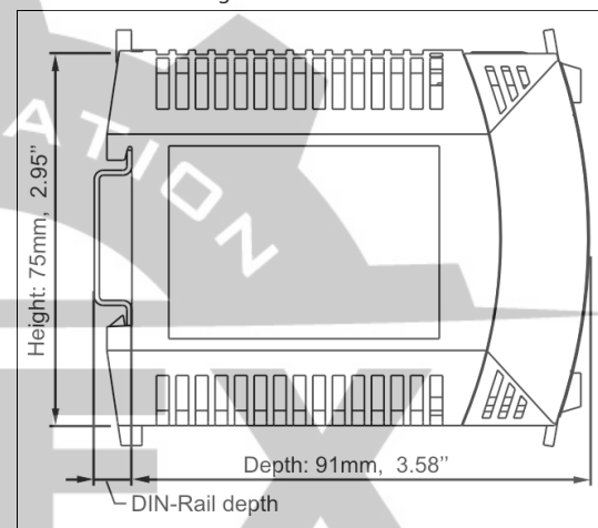
Fig. 15-2 Side view
