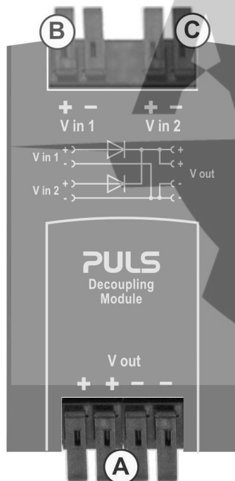
Fig. 8-1 Front side
