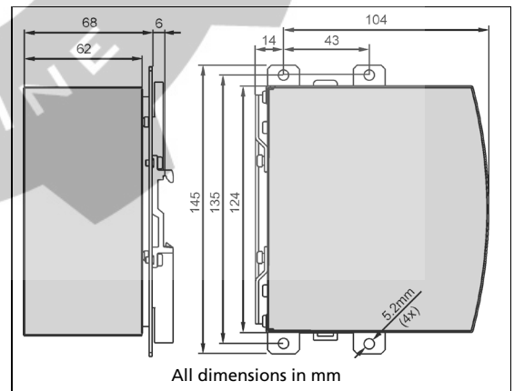
Fig. 21-11 Hole pattern
