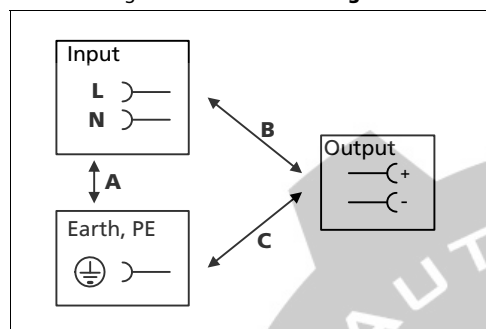
Fig. 17-1 Dielectric strength
