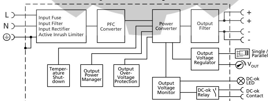
Fig. 11-1 Functional diagram
