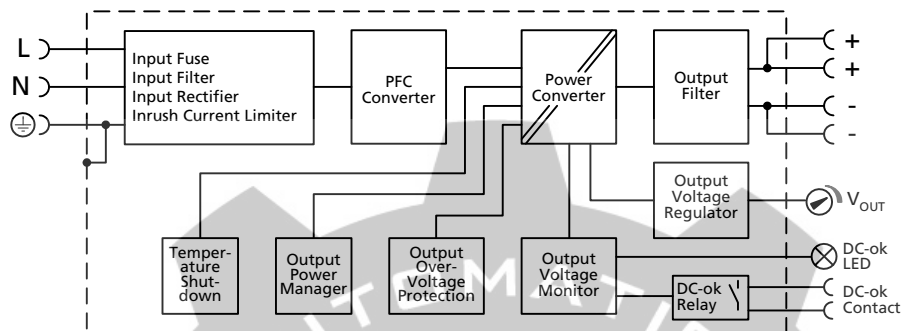
Fig. 10-1 Functional diagram
