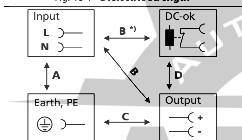
Fig. 18-1 Dielectric strength
