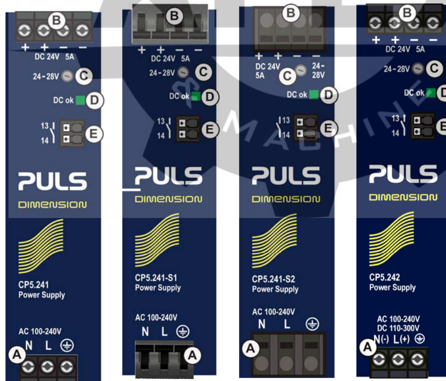
Fig. 11-1 Front side
