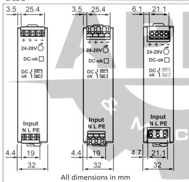
Fig. 21-1 Front view
