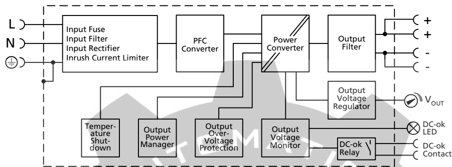
Fig. 10-1 Functional diagram
