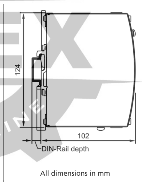
Fig. 21-2 Side view
