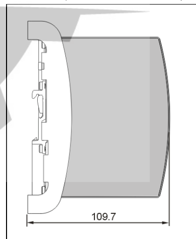
Fig. 22-6 Wall/panel mounting, side view (Picture shows the CP5.241)
