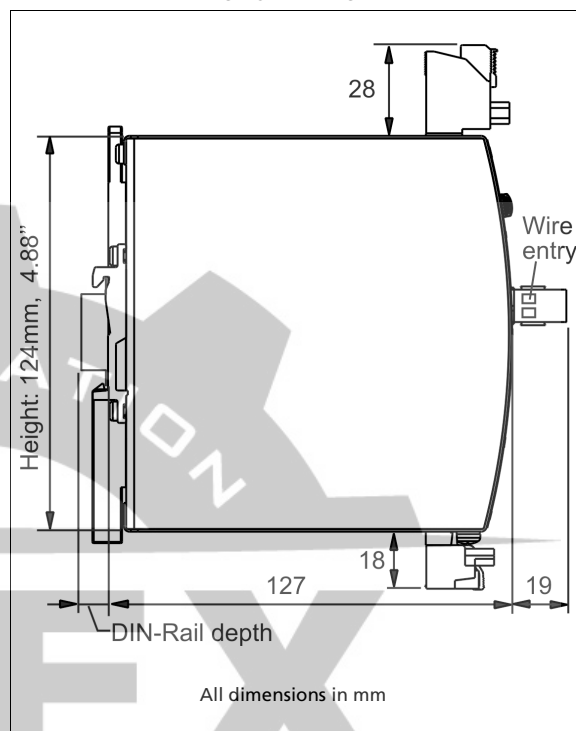
Fig. 22-4 Side view CP20.241-R2, CP20.242-R2, CP20.241-R2-C1
