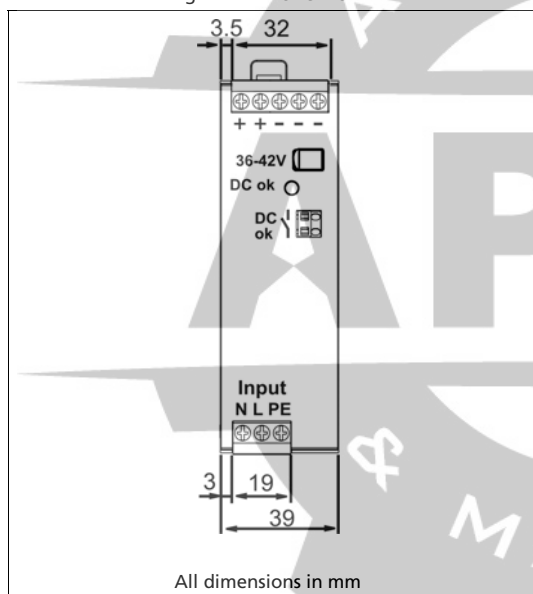
Fig. 22-1 Front view
