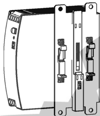
Side mounting with DIN-rail brackets
