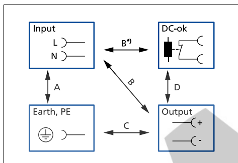
Fig. 20-1: Dielectric strength
