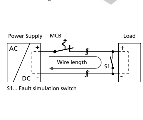
Fig. 24-4 Test circuit
