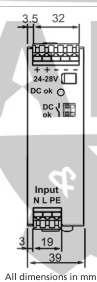
Fig. 22-2 Front view CP10.241-S1
