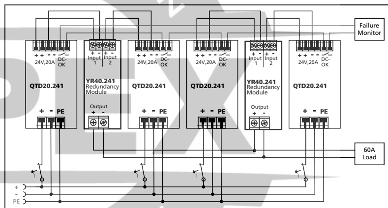
Fig. 21-8 Typical N+1 Redundant configuration for 60A with two dual redundancy modules and four DC/DC converters
