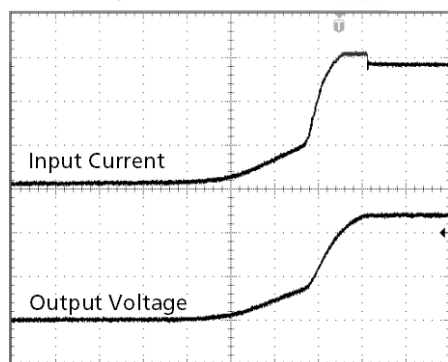
Fig. 4-2 Soft-start behavior
