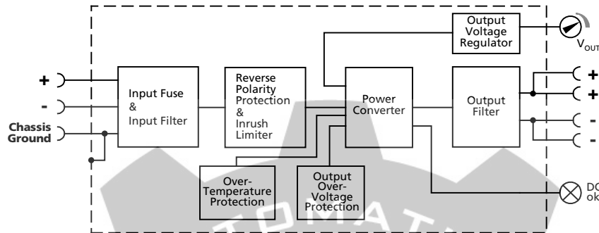
Fig. 8-1 Functional diagram
