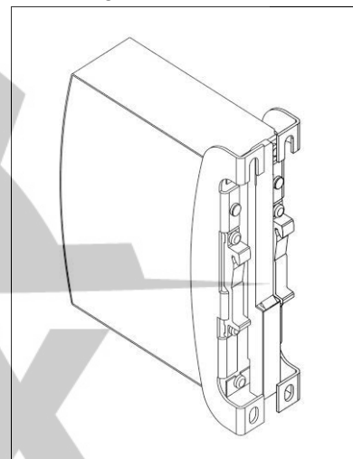
Fig. 20-3 Isometric view
