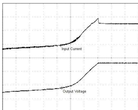
Fig. 4-2 Soft-start behavior
