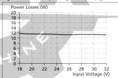
Fig. 7-4 Losses vs. input voltage at 5.1V, 10A, typ.
