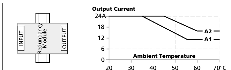
Fig. 18-11 Mounting Orientation E (Horizontal ccw)
