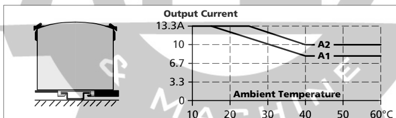
Fig. 25-4 Mounting Orientation C (Table-top mounting)
