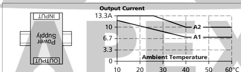
Fig. 25-3 Mounting Orientation B (Upside down)
