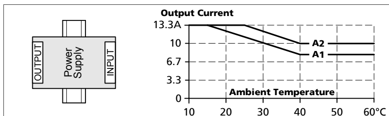
Fig. 25-6 Mounting Orientation E (Horizontal ccw)
