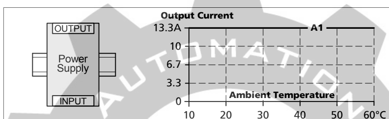
Fig. 25-2 Mounting Orientation A Standard Orientation
