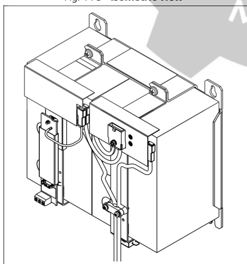
Fig. 14-3 Isometric view
