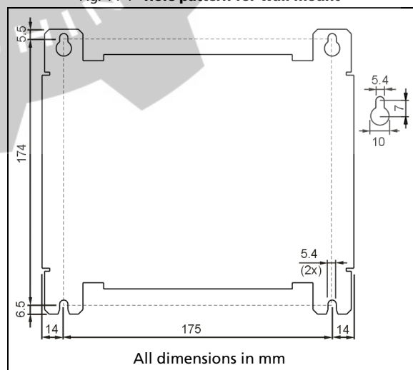
Fig. 14-4 Hole pattern for wall mount
