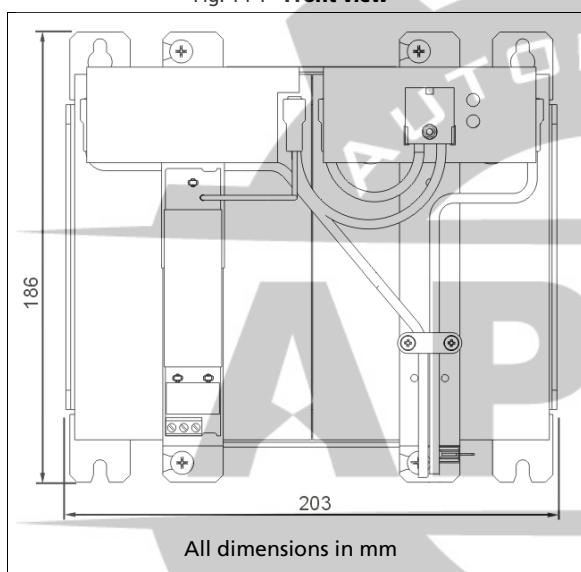
Fig. 14-1 Front view
