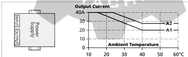
Fig. 26-13 Mounting Orientation D (Horizontal cw)
