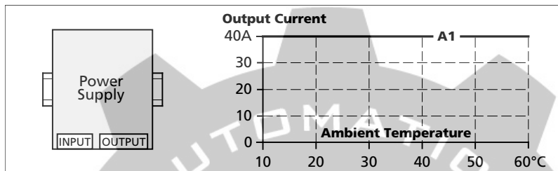
Fig. 26-10 Mounting Orientation A (Standard orientation)
