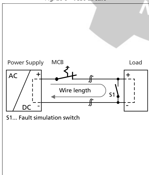
Fig. 26-9 Test circuit
