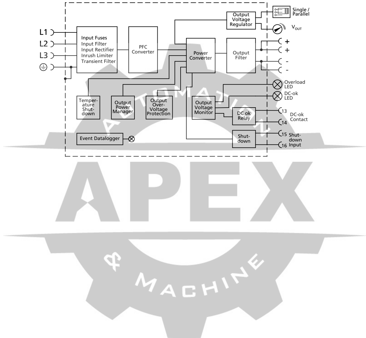
Fig. 14-1 Functional diagram
