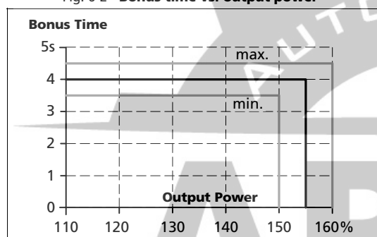
Fig. 6-2 Bonus time vs. output power
