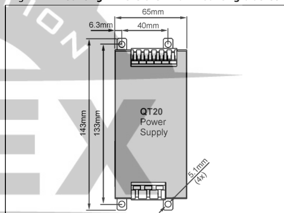
Fig. 21-2 Mounting Dimensions - Wall mounting bracket
