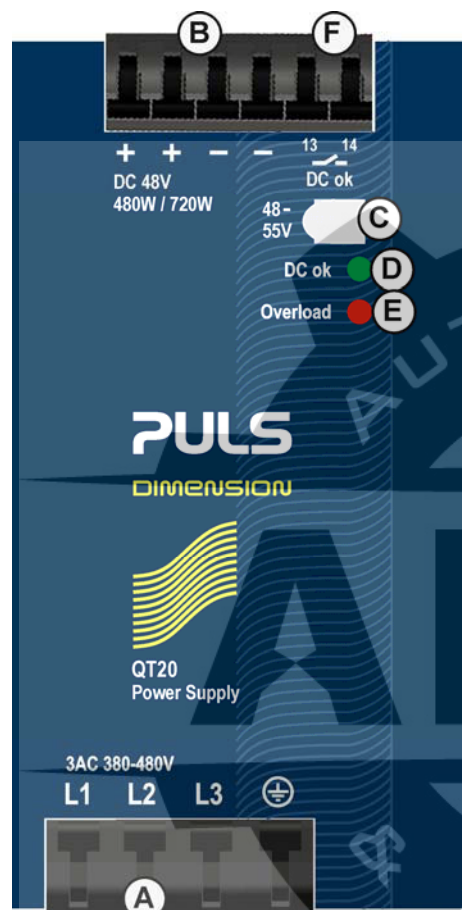
Fig. 13-1 Front side
