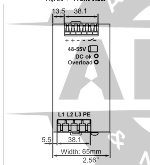
Fig. 20-1 Front view
