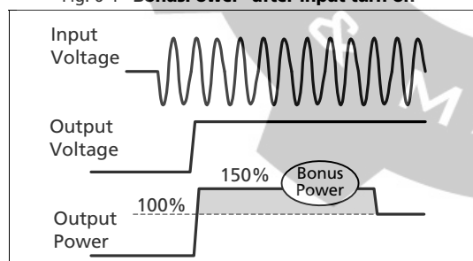
Fig. 6-4 BonusPower® after input turn-on
