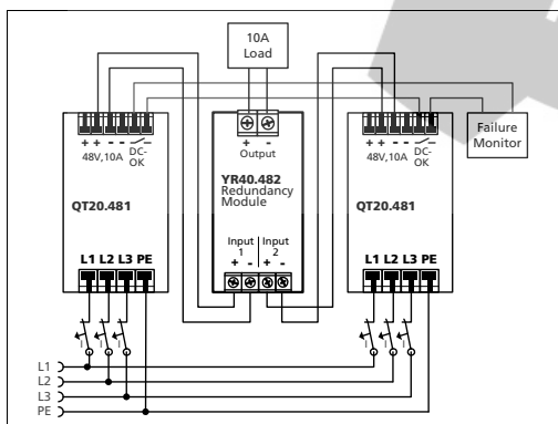
Fig. 21-6 Typical 1+1 Redundant configuration for 10A with one dual redundancy module and two power supplies
