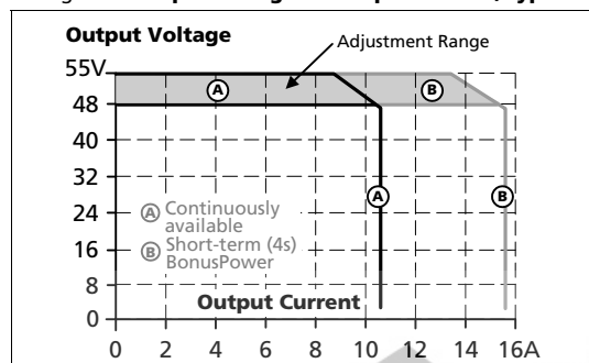
Fig. 6-1 Output voltage vs. output current, typ.
