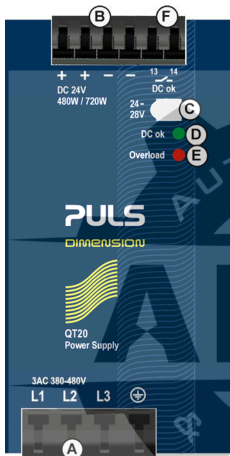
Fig. 13-1 Front side
