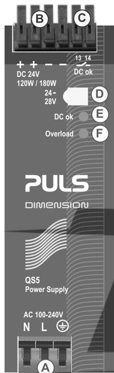
Fig. 13-1 Front side
