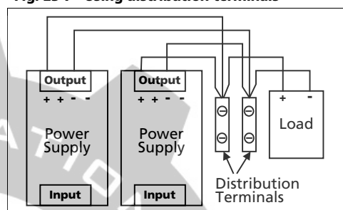
Fig. 23-7 Using distribution terminals
