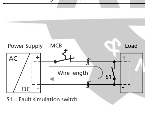
Fig. 4-5 Test circuit
