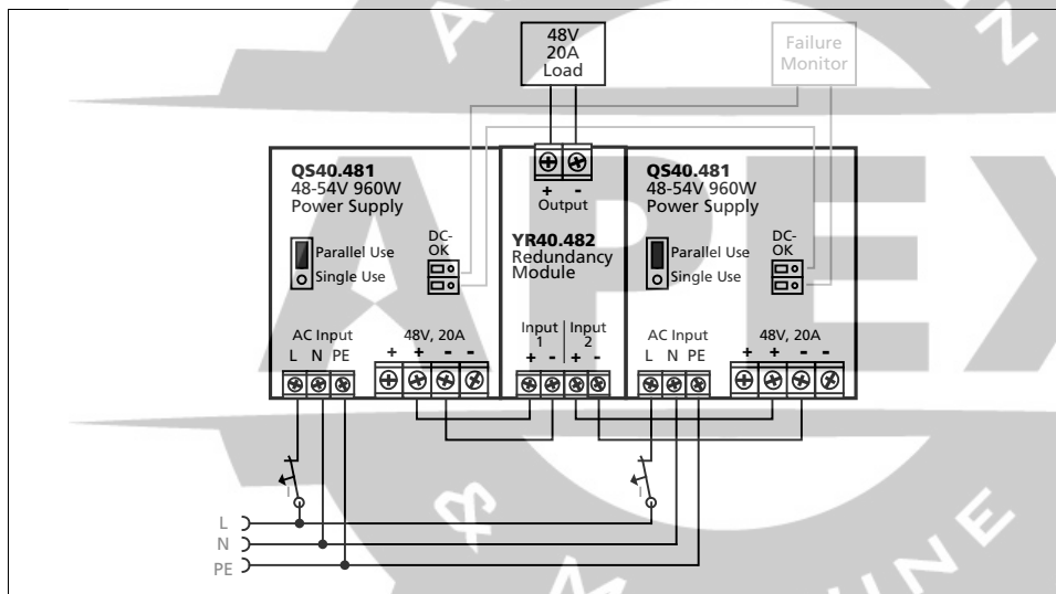
Fig. 3-1 Typical 1+1 Redundant configuration for 20A with a dual redundancy module
