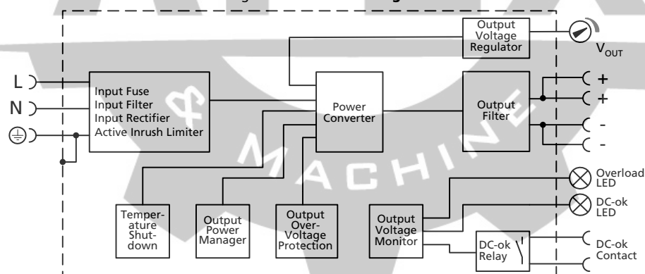
Fig. 11-1 Functional diagram
