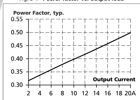
Fig. 3-4 Power factor vs. output load
