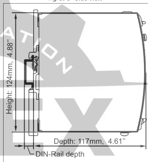
Fig. 20-2 Side view
