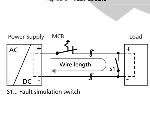
Fig. 22-5 Test circuit
