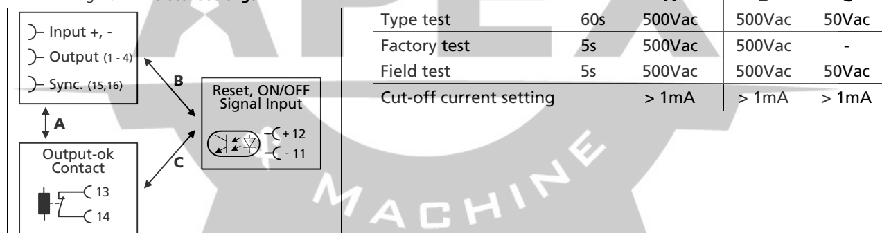
Fig. 20-1 Dielectric strength
