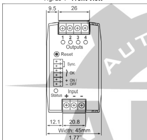
Fig. 25-1 Front view
