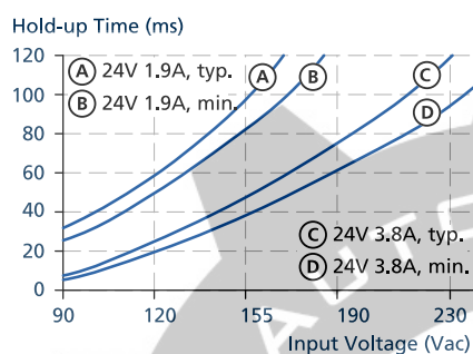
Fig. 7-1: Hold-up time vs. input voltage
