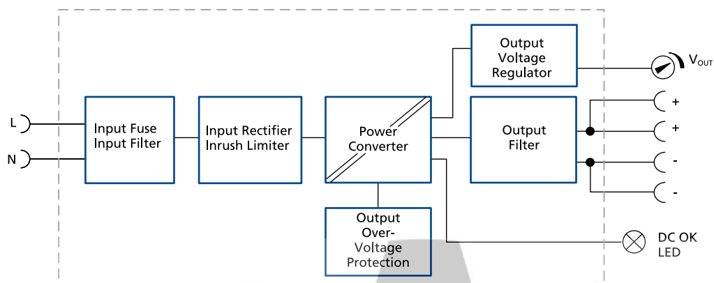
Fig. 11-1: Functional diagram
