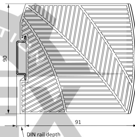
Fig. 20-2: Side view
