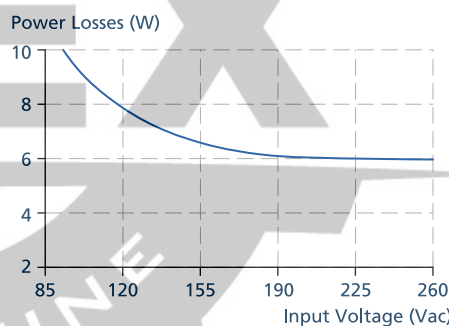
Fig. 8-4: Losses vs. input voltage at 24V, 3.8A, typ.
