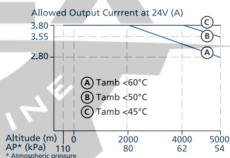
Fig. 15-2: Output power vs. altitude
