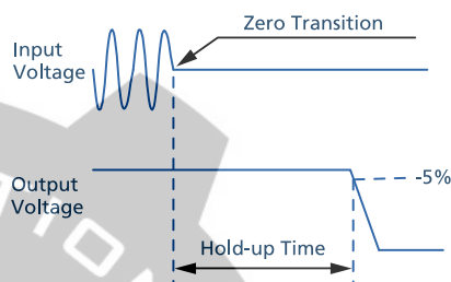
Fig. 7-2: Shut-down behaviour, definitions
