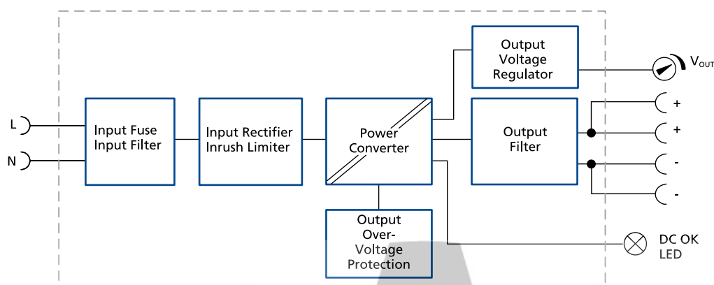
Fig. 11-1: Functional diagram
