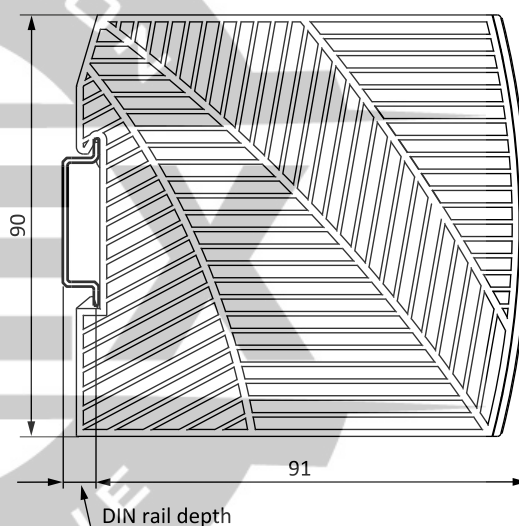
Fig. 20-2: Side view
