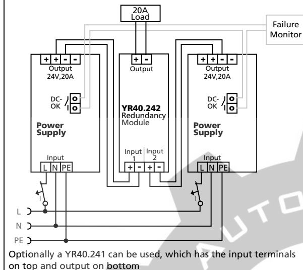
Fig. 23-1 1+1 Redundant wiring with 1 YR40.242
