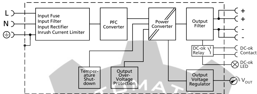
Fig. 10-1 Functional diagram
