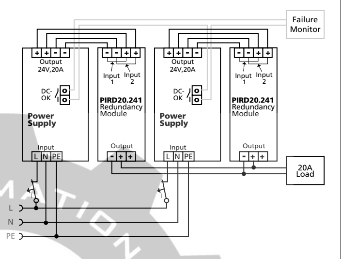
Fig. 23-2 1+1 Redundant wiring with 2 PIRD20.241
