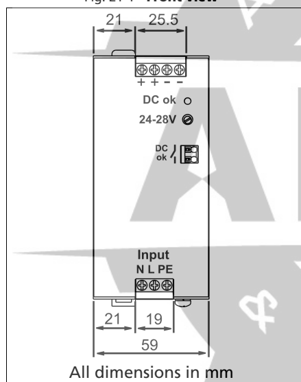
Fig. 21-1 Front view
