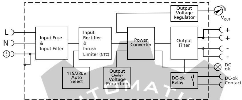
Fig. 10-1 Functional diagram
