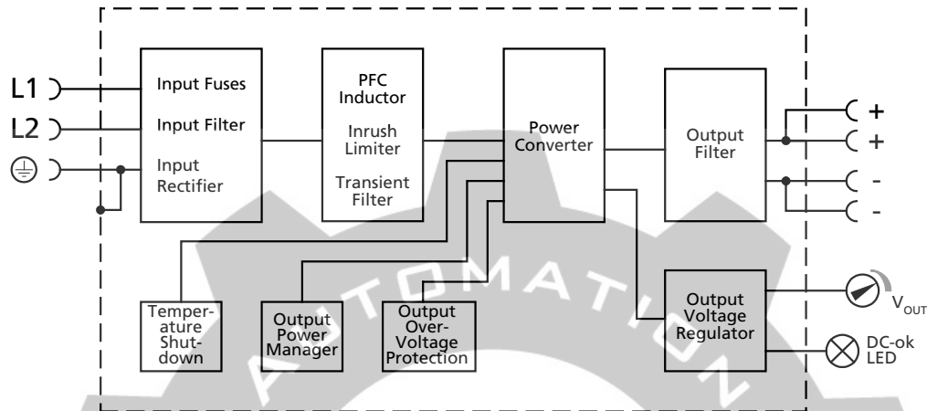
Fig. 9-1 Functional diagram
