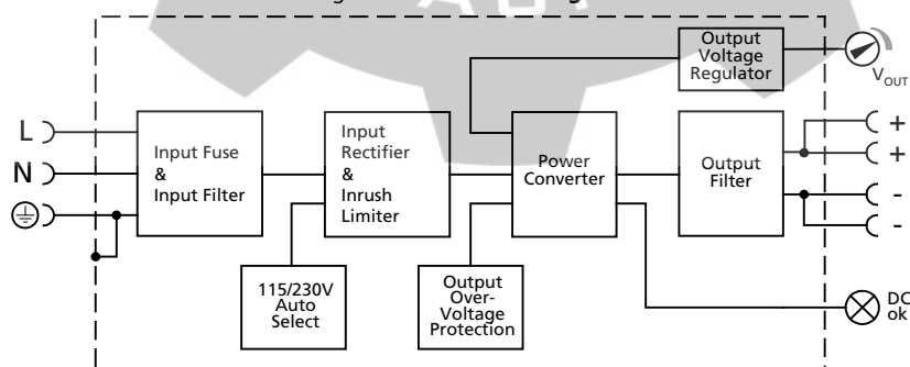
Fig. 10-1 Functional diagram
