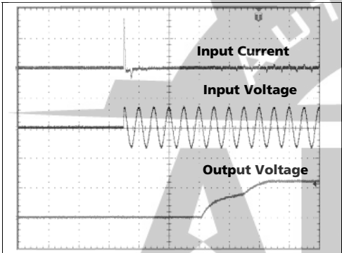
Fig. 5-1 Typical input inrush current behavior
