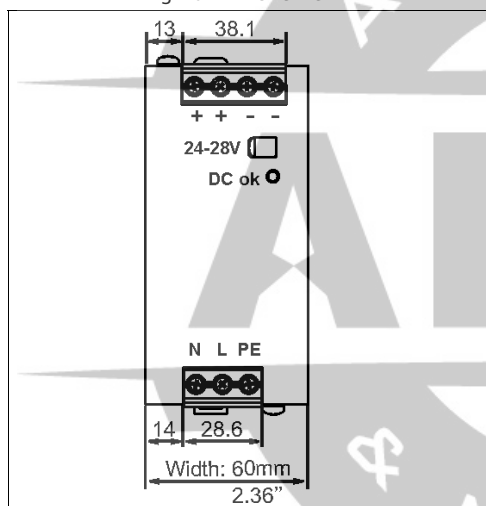
Fig. 20-1 Front view
