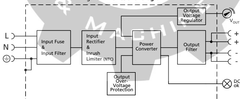
Fig. 10-1 Functional diagram
