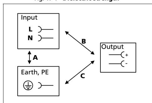
Fig. 17-1 Dielectric strength
