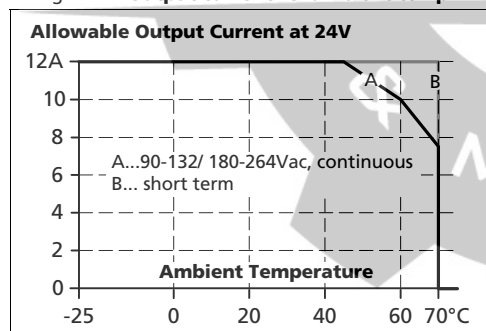
Fig. 14-1 Output current vs. ambient temp.
