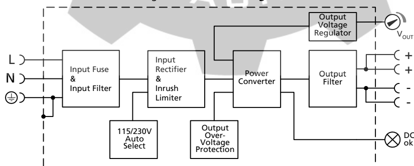
Fig. 10-1 Functional diagram
