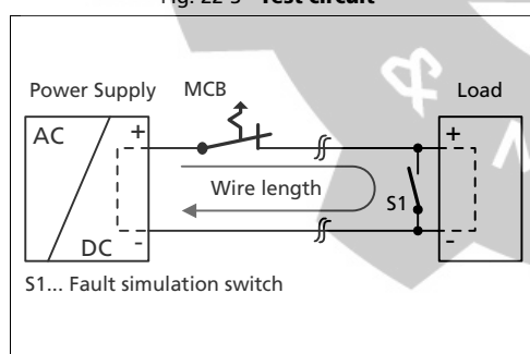
Fig. 22-3 Test circuit
