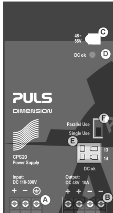
Fig. 13-1 Front side
