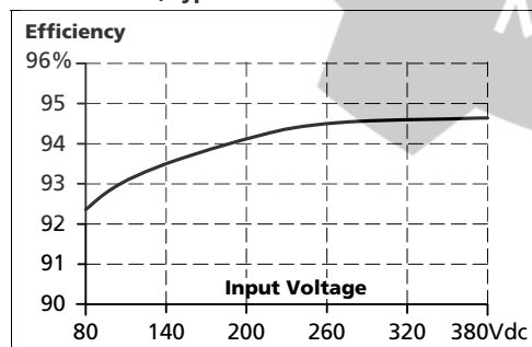
Fig. 9-3 Efficiency vs. input voltage at 48V, 10A, typ.
