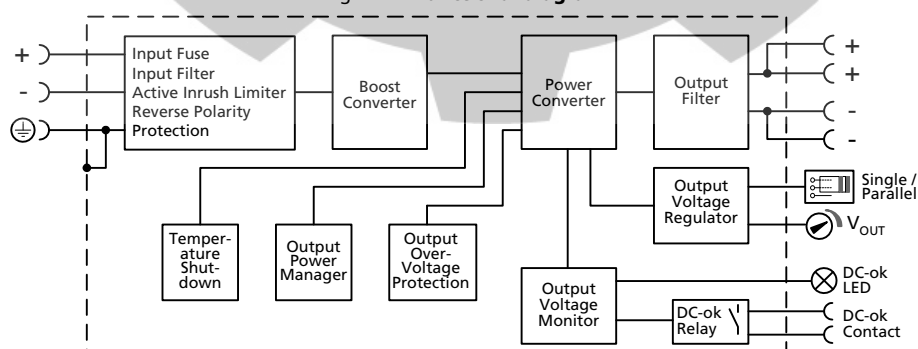
Fig. 11-1 Functional diagram
