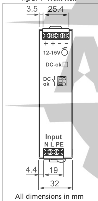
Fig. 21-1 Front view
