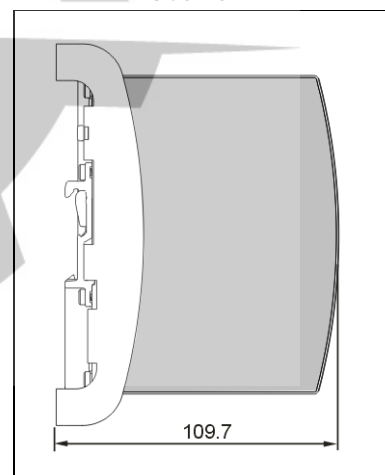
Fig. 22-6 Wall/panel mounting, side view
