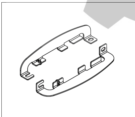
Fig. 23-2 ZM10.Wall Wall mounting bracket*)
