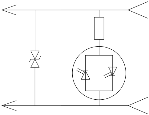
LED W/ DUAL ZENOR DIODES
